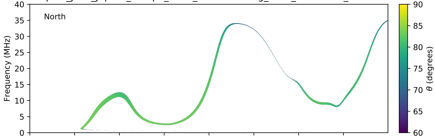
expres_juno_jupiter_europa_isaac_lossc-wid1deg_3kev_20180103_v01.cdf
