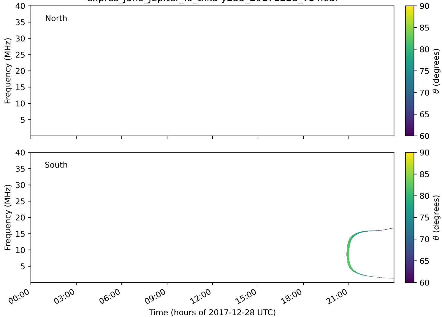
expres_juno_jupiter_io_txka-y235_20171228_v14.cdf
