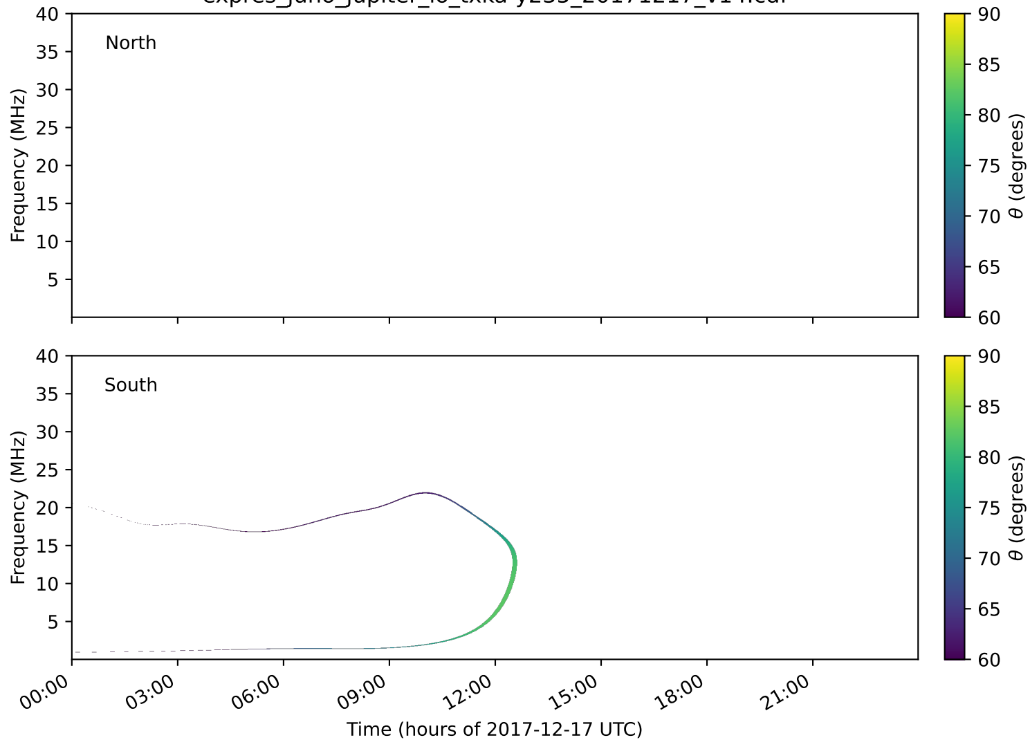
expres_juno_jupiter_io_txka-y235_20171217_v14.cdf
