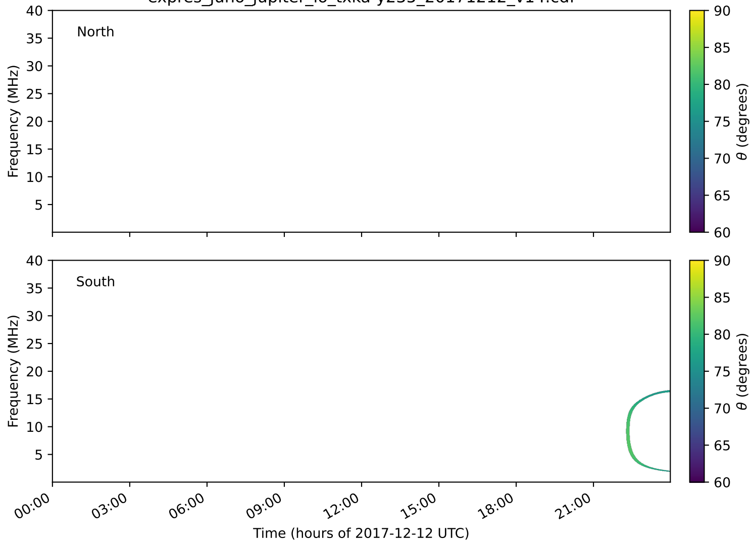
expres_juno_jupiter_io_txka-y235_20171212_v14.cdf
