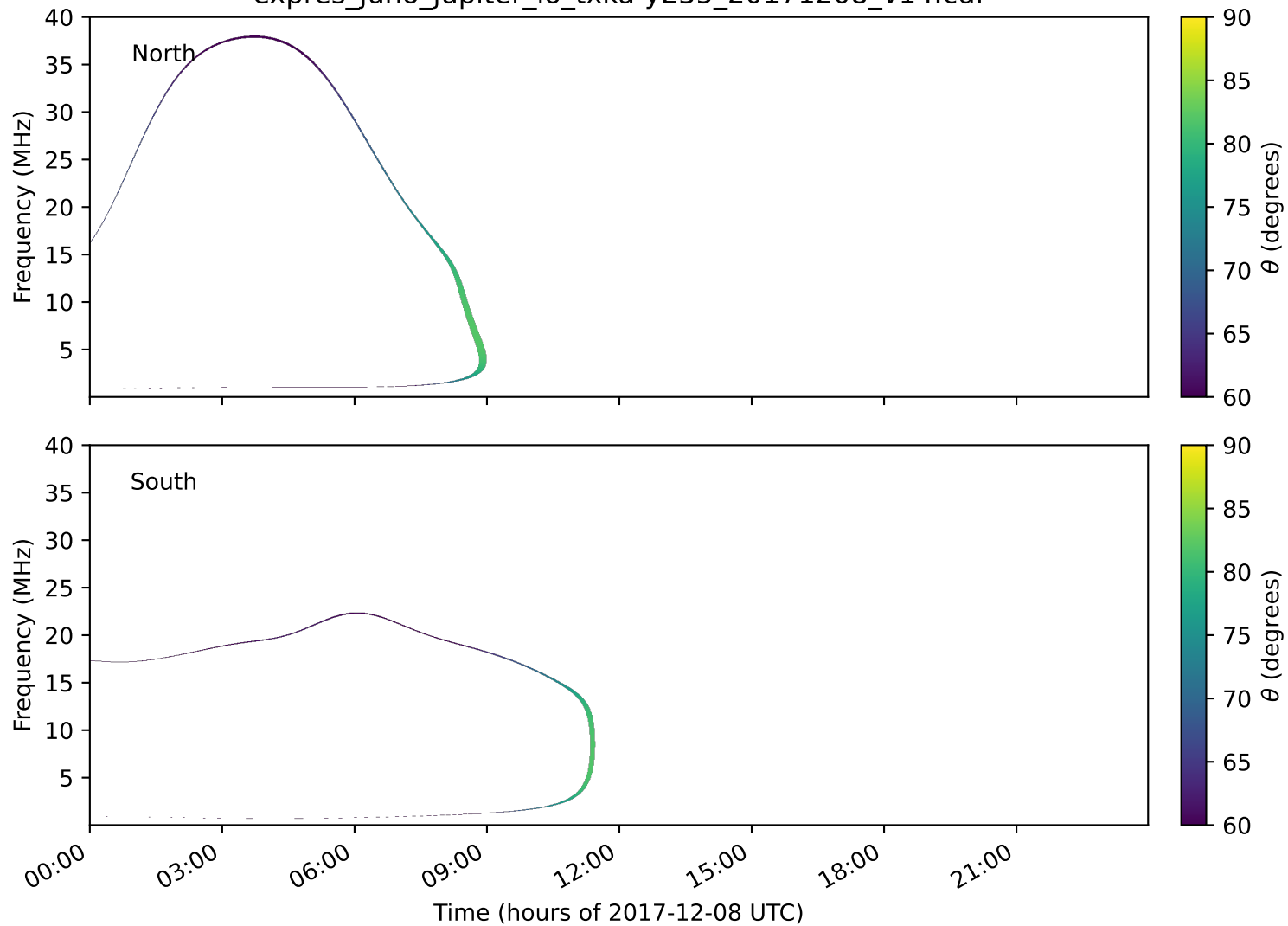
expres_juno_jupiter_io_txka-y235_20171208_v14.cdf
