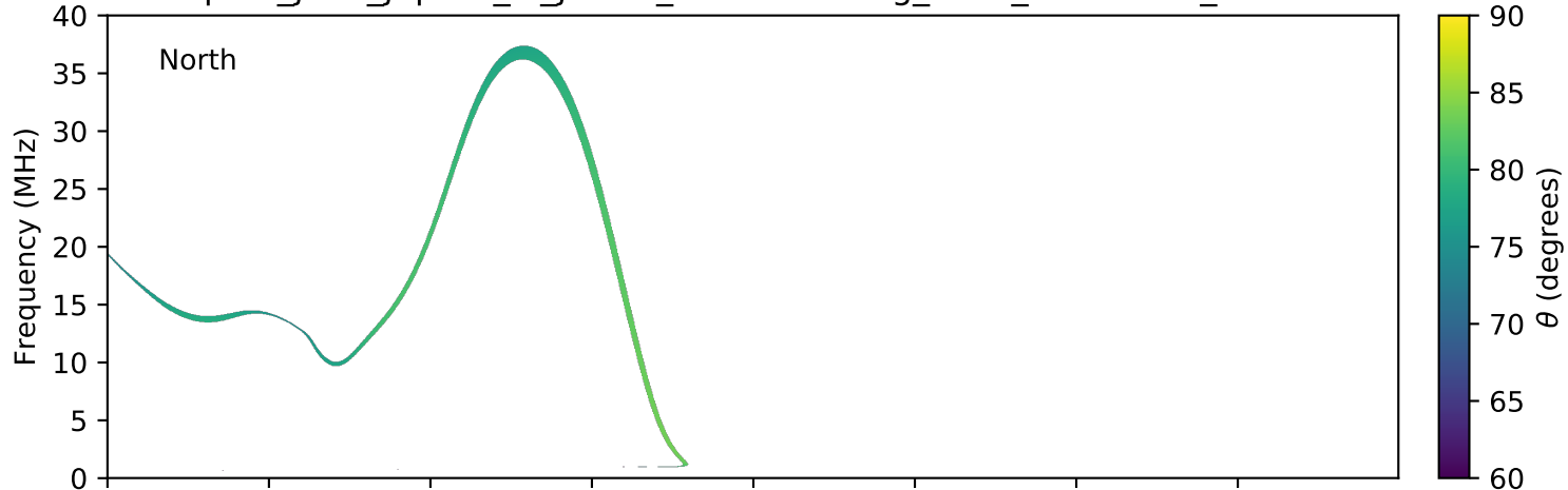
expres_juno_jupiter_io_jrm09_lossc-wid1deg_3kev_20171231_v01.cdf
