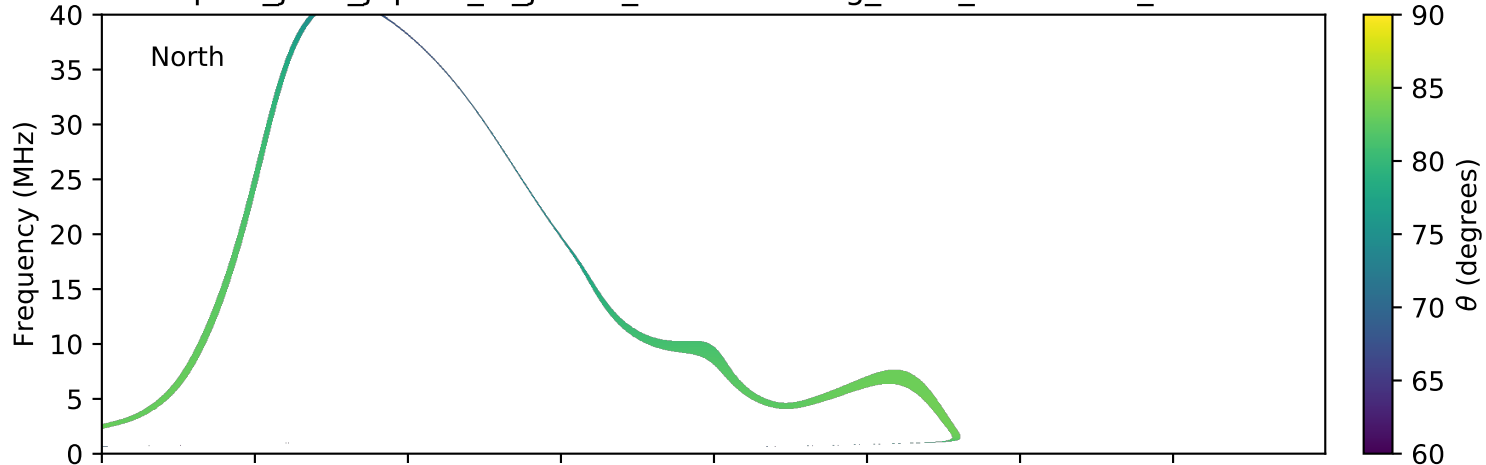
expres_juno_jupiter_io_jrm09_lossc-wid1deg_3kev_20171229_v01.cdf
