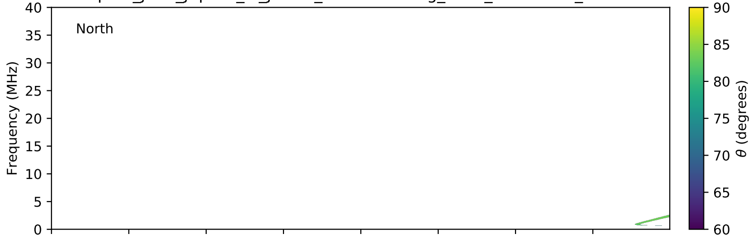
expres_juno_jupiter_io_jrm09_lossc-wid1deg_3kev_20171228_v01.cdf
