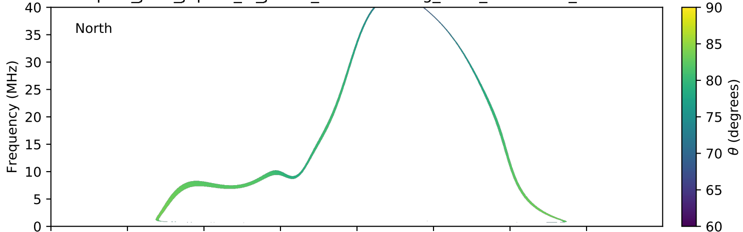
expres_juno_jupiter_io_jrm09_lossc-wid1deg_3kev_20171227_v01.cdf
