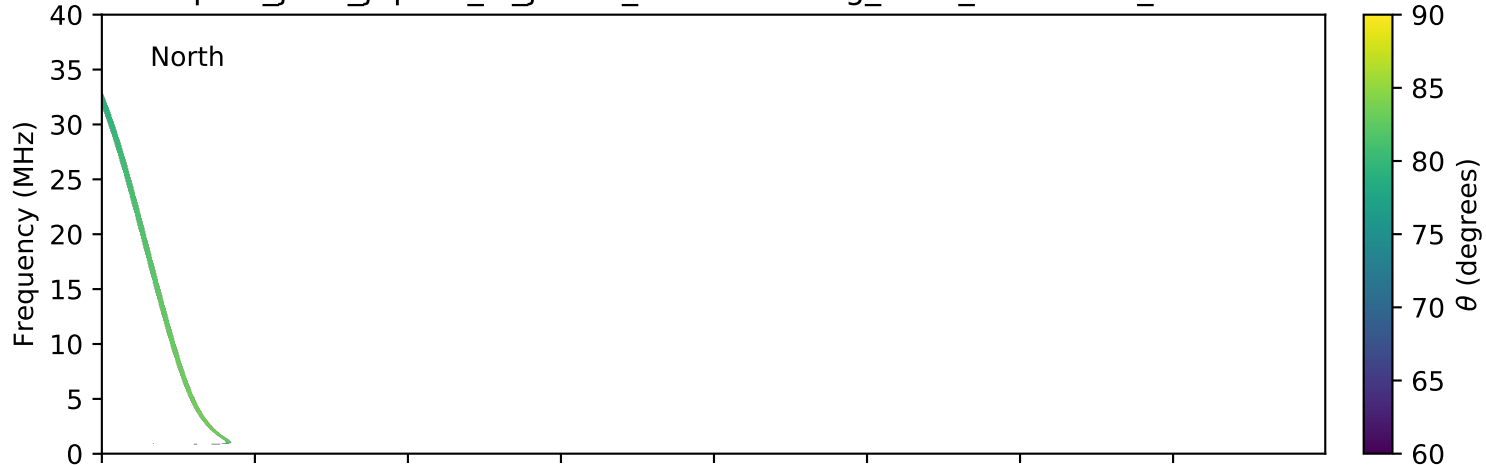
expres_juno_jupiter_io_jrm09_lossc-wid1deg_3kev_20171226_v01.cdf
