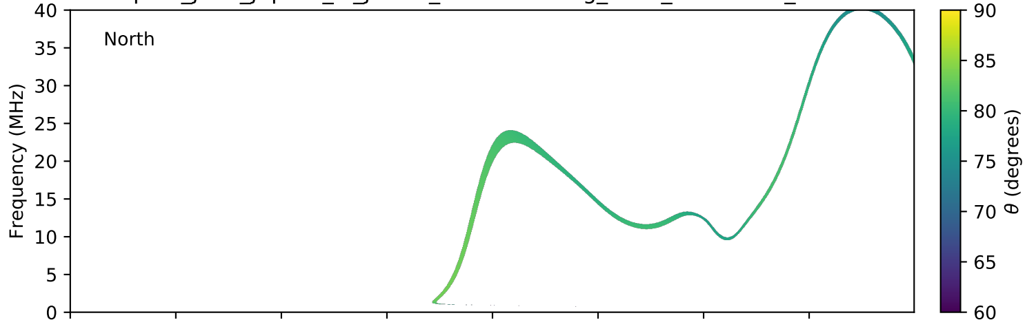
expres_juno_jupiter_io_jrm09_lossc-wid1deg_3kev_20171225_v01.cdf
