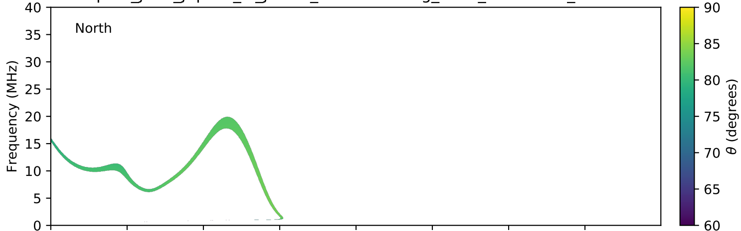
expres_juno_jupiter_io_jrm09_lossc-wid1deg_3kev_20171224_v01.cdf
