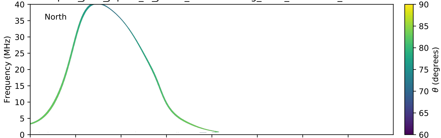
expres_juno_jupiter_io_jrm09_lossc-wid1deg_3kev_20171222_v01.cdf
