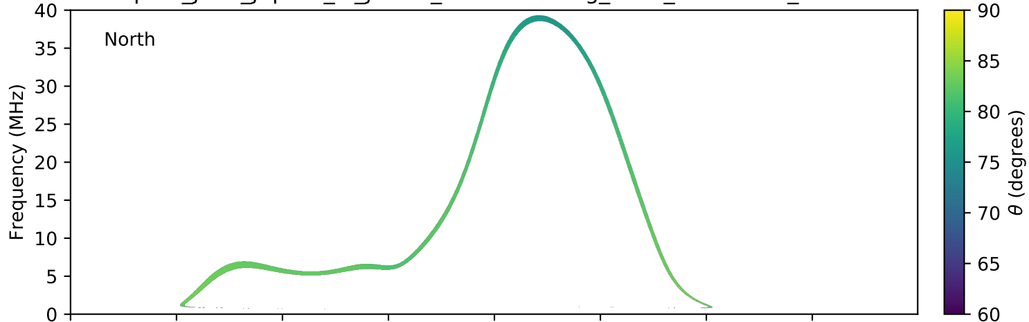
expres_juno_jupiter_io_jrm09_lossc-wid1deg_3kev_20171220_v01.cdf
