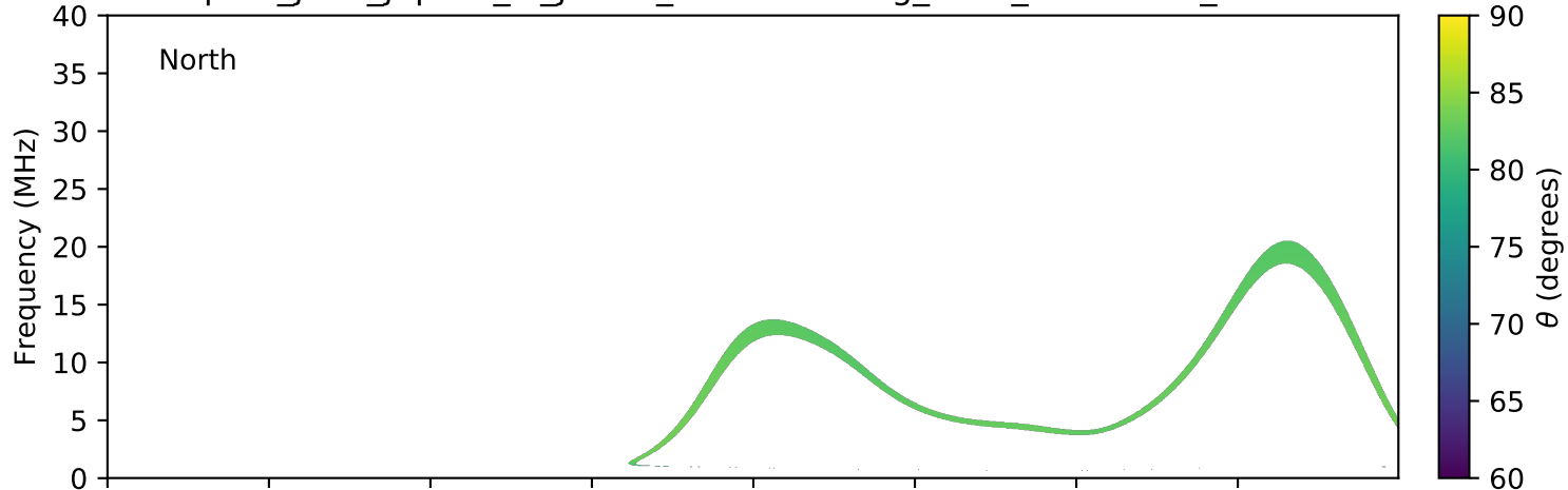
expres_juno_jupiter_io_jrm09_lossc-wid1deg_3kev_20171218_v01.cdf
