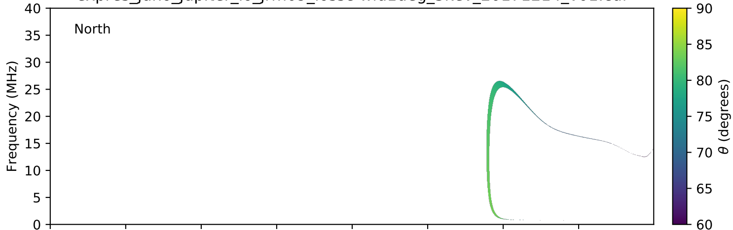
expres_juno_jupiter_io_jrm09_lossc-wid1deg_3kev_20171214_v01.cdf
