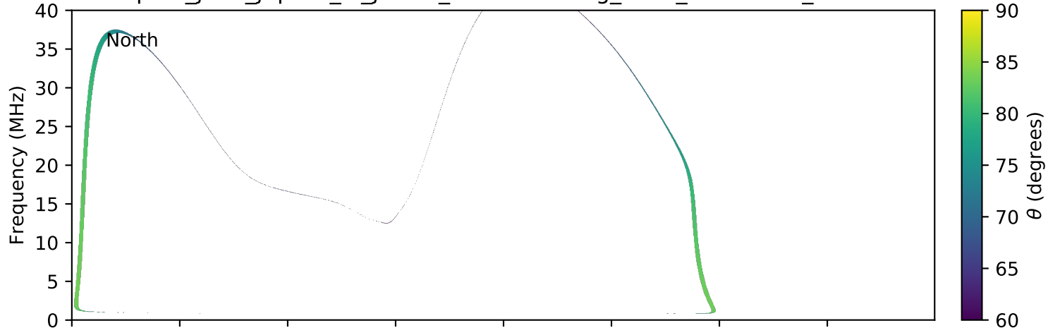
expres_juno_jupiter_io_jrm09_lossc-wid1deg_3kev_20171213_v01.cdf
