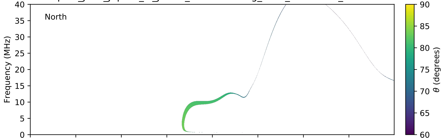
expres_juno_jupiter_io_jrm09_lossc-wid1deg_3kev_20171209_v01.cdf
