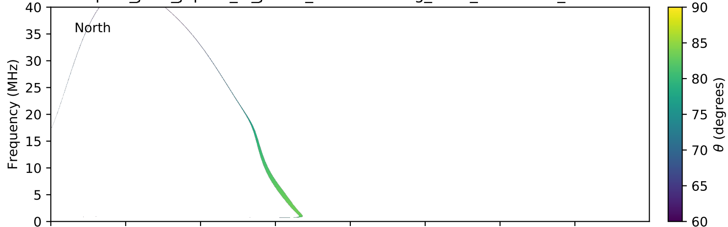
expres_juno_jupiter_io_jrm09_lossc-wid1deg_3kev_20171208_v01.cdf
