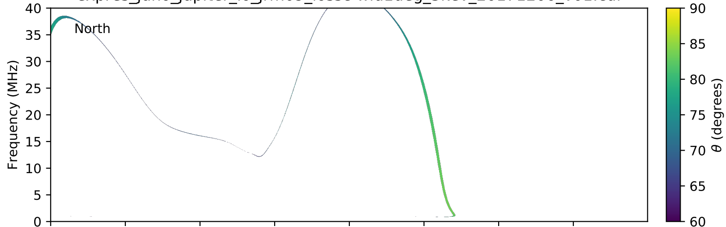
expres_juno_jupiter_io_jrm09_lossc-wid1deg_3kev_20171206_v01.cdf
