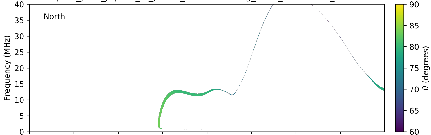
expres_juno_jupiter_io_jrm09_lossc-wid1deg_3kev_20171202_v01.cdf
