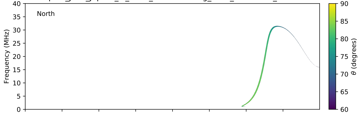
expres_juno_jupiter_io_isaac_lossc-wid1deg_3kev_20171230_v01.cdf
