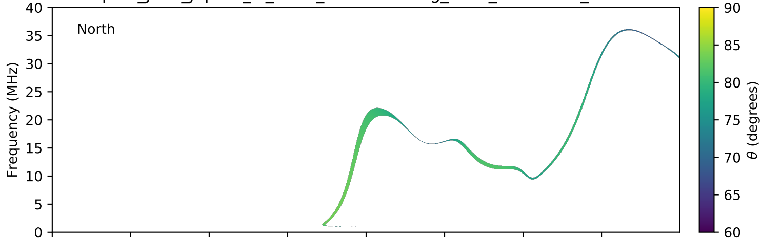
expres_juno_jupiter_io_isaac_lossc-wid1deg_3kev_20171225_v01.cdf
