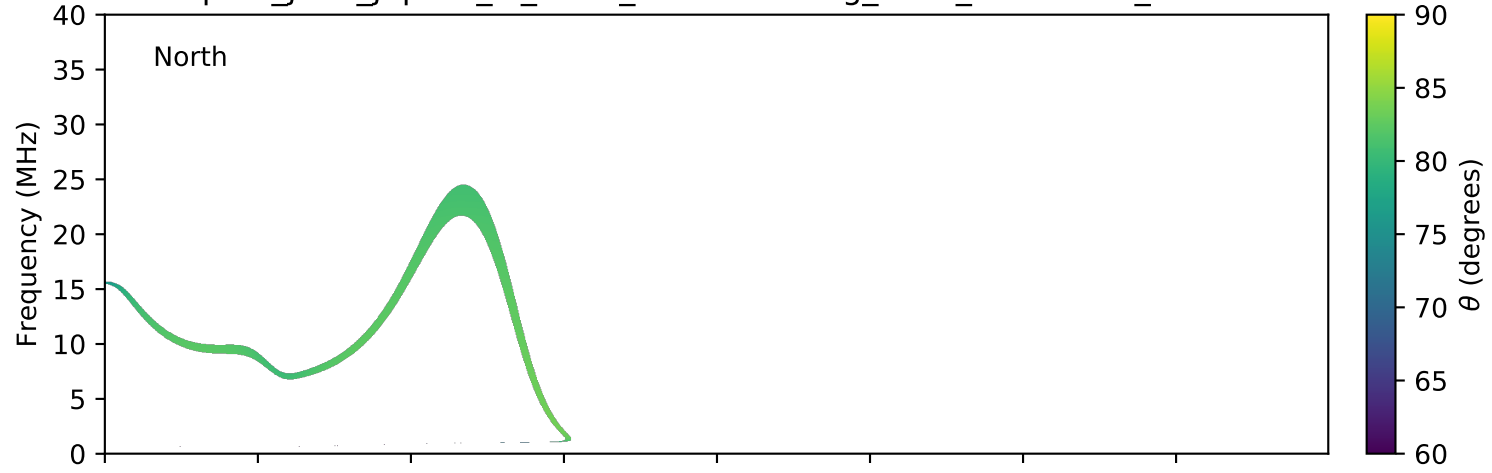
expres_juno_jupiter_io_isaac_lossc-wid1deg_3kev_20171224_v01.cdf
