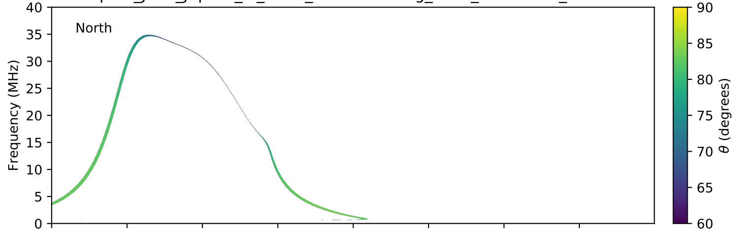
expres_juno_jupiter_io_isaac_lossc-wid1deg_3kev_20171222_v01.cdf
