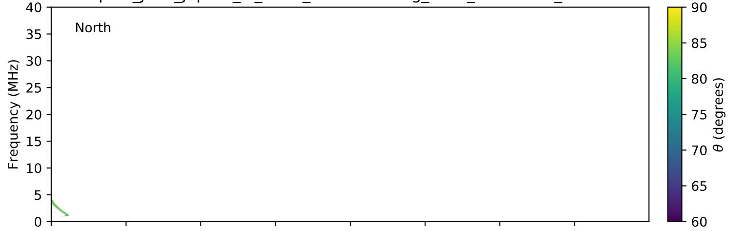
expres_juno_jupiter_io_isaac_lossc-wid1deg_3kev_20171219_v01.cdf
