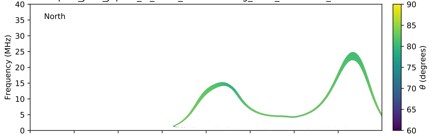
expres_juno_jupiter_io_isaac_lossc-wid1deg_3kev_20171218_v01.cdf
