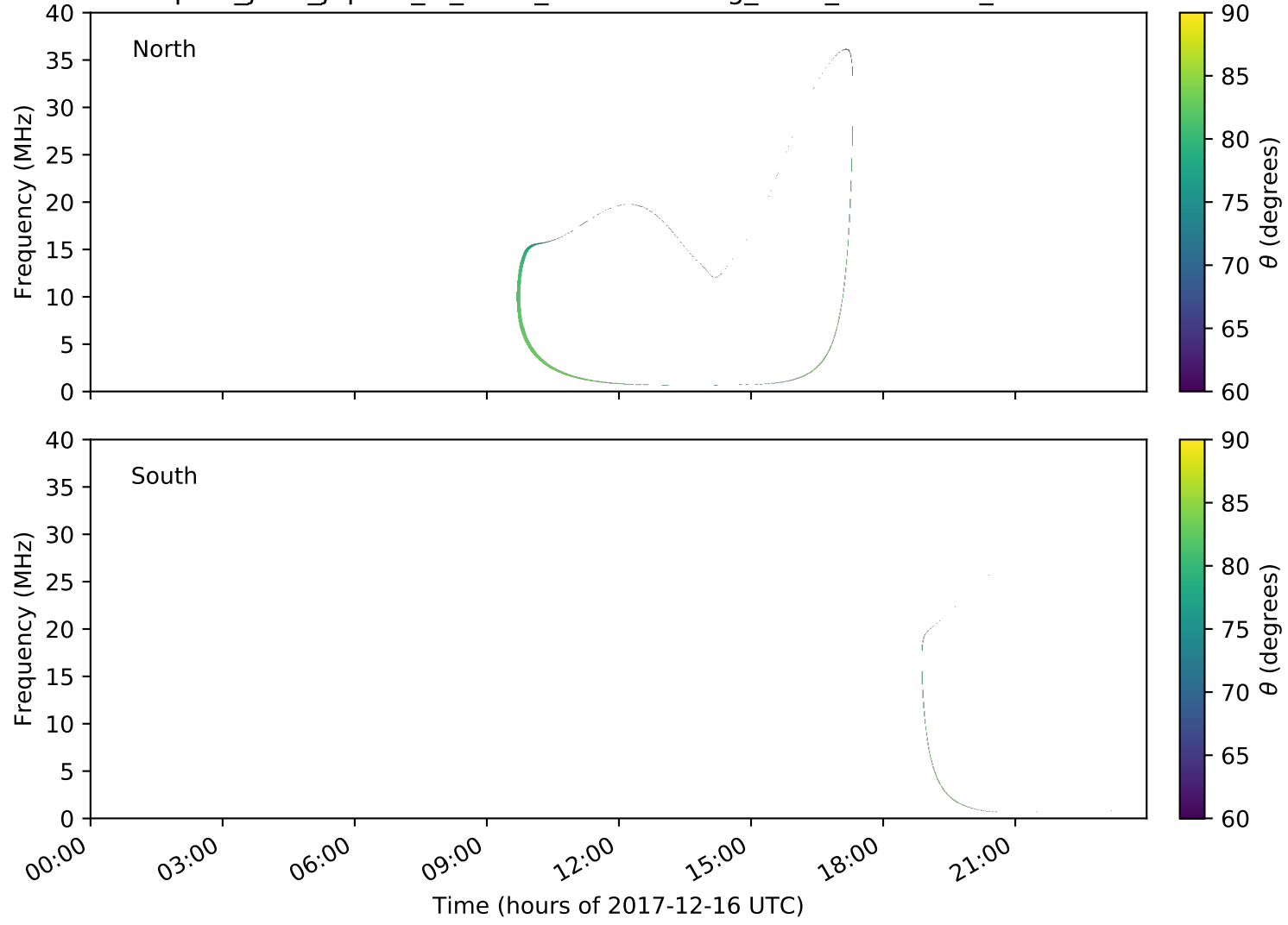
expres_juno_jupiter_io_isaac_lossc-wid1deg_3kev_20171216_v01.cdf
