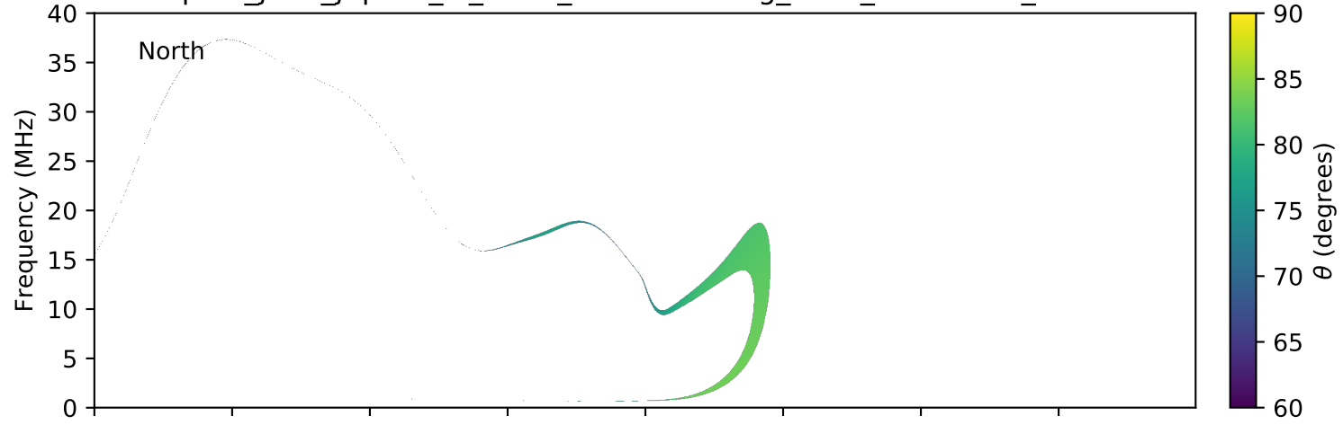
expres_juno_jupiter_io_isaac_lossc-wid1deg_3kev_20171215_v01.cdf
