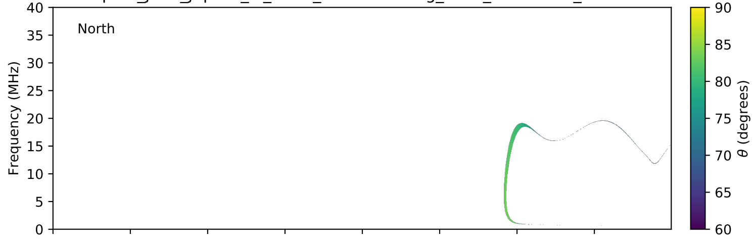
expres_juno_jupiter_io_isaac_lossc-wid1deg_3kev_20171214_v01.cdf
