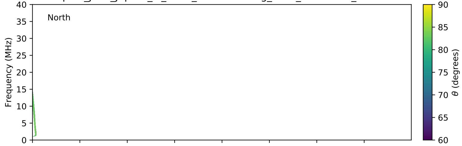
expres_juno_jupiter_io_isaac_lossc-wid1deg_3kev_20171212_v01.cdf
