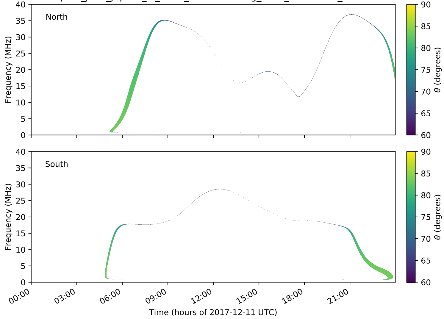
expres_juno_jupiter_io_isaac_lossc-wid1deg_3kev_20171211_v01.cdf
