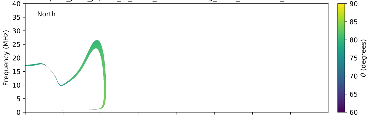
expres_juno_jupiter_io_isaac_lossc-wid1deg_3kev_20171210_v01.cdf
