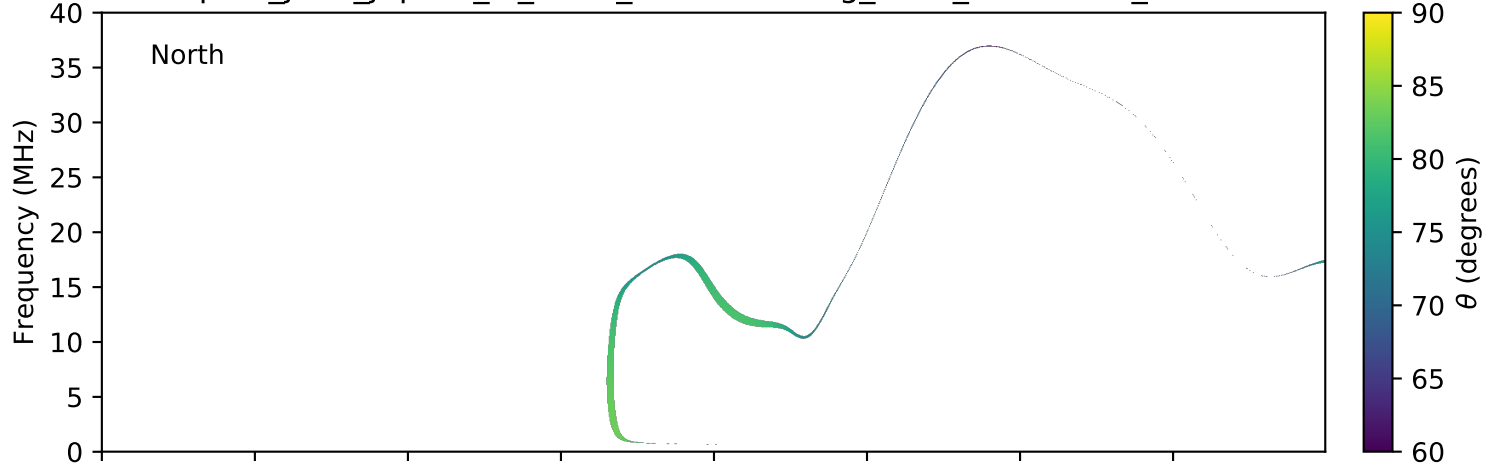
expres_juno_jupiter_io_isaac_lossc-wid1deg_3kev_20171209_v01.cdf
