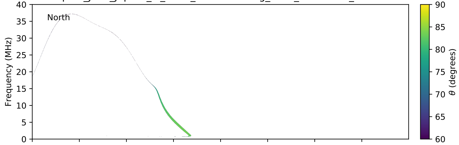
expres_juno_jupiter_io_isaac_lossc-wid1deg_3kev_20171208_v01.cdf
