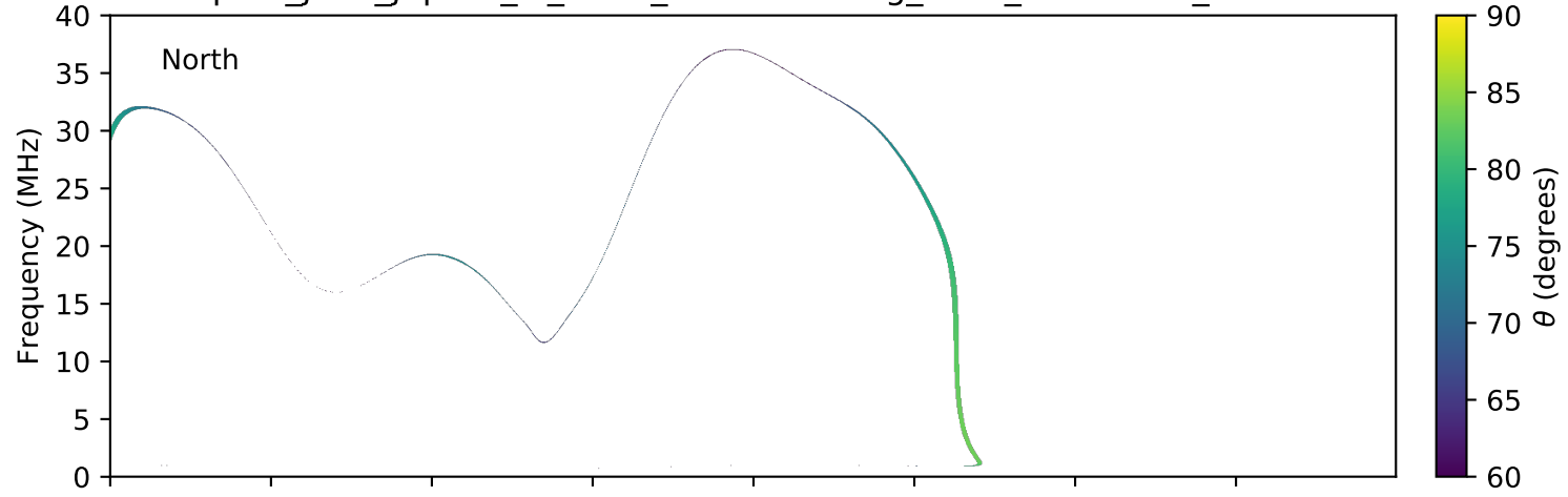
expres_juno_jupiter_io_isaac_lossc-wid1deg_3kev_20171206_v01.cdf
