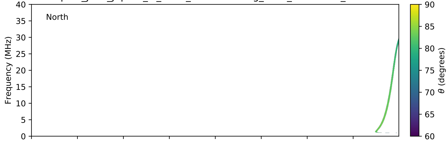
expres_juno_jupiter_io_isaac_lossc-wid1deg_3kev_20171205_v01.cdf
