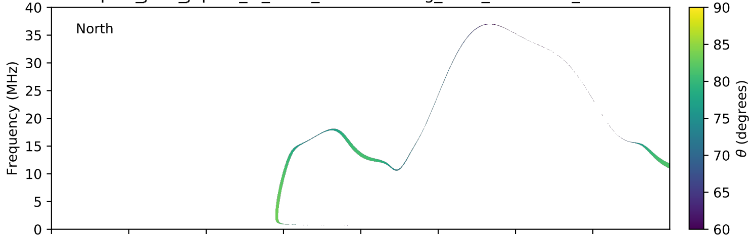
expres_juno_jupiter_io_isaac_lossc-wid1deg_3kev_20171202_v01.cdf
