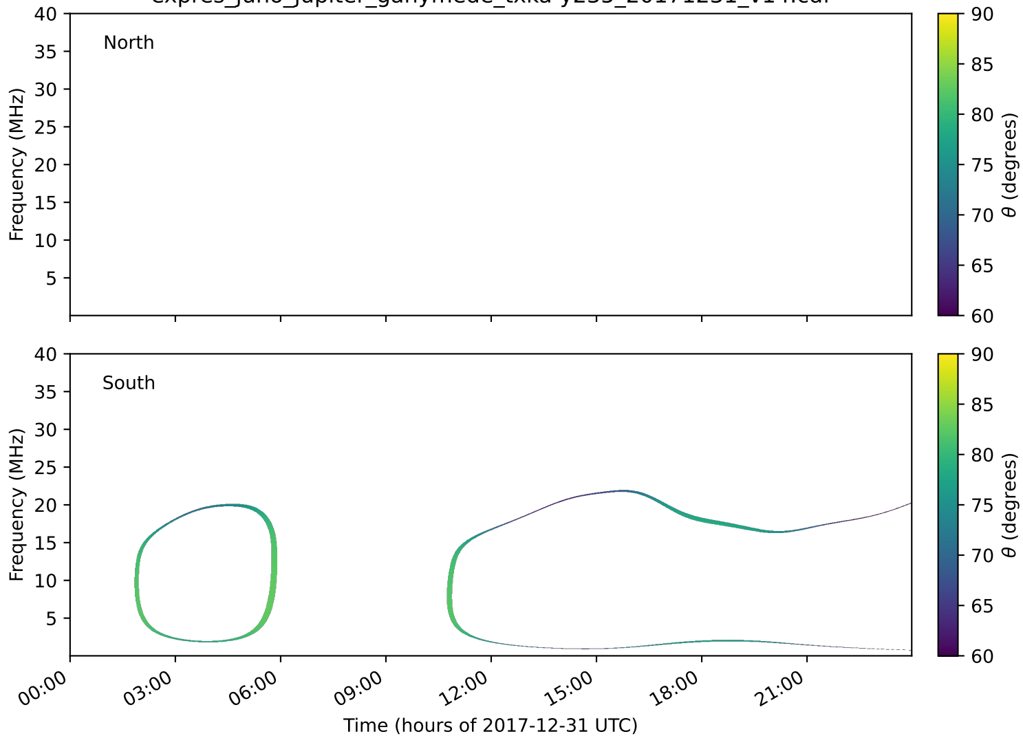
expres_juno_jupiter_ganymede_txka-y235_20171231_v14.cdf
