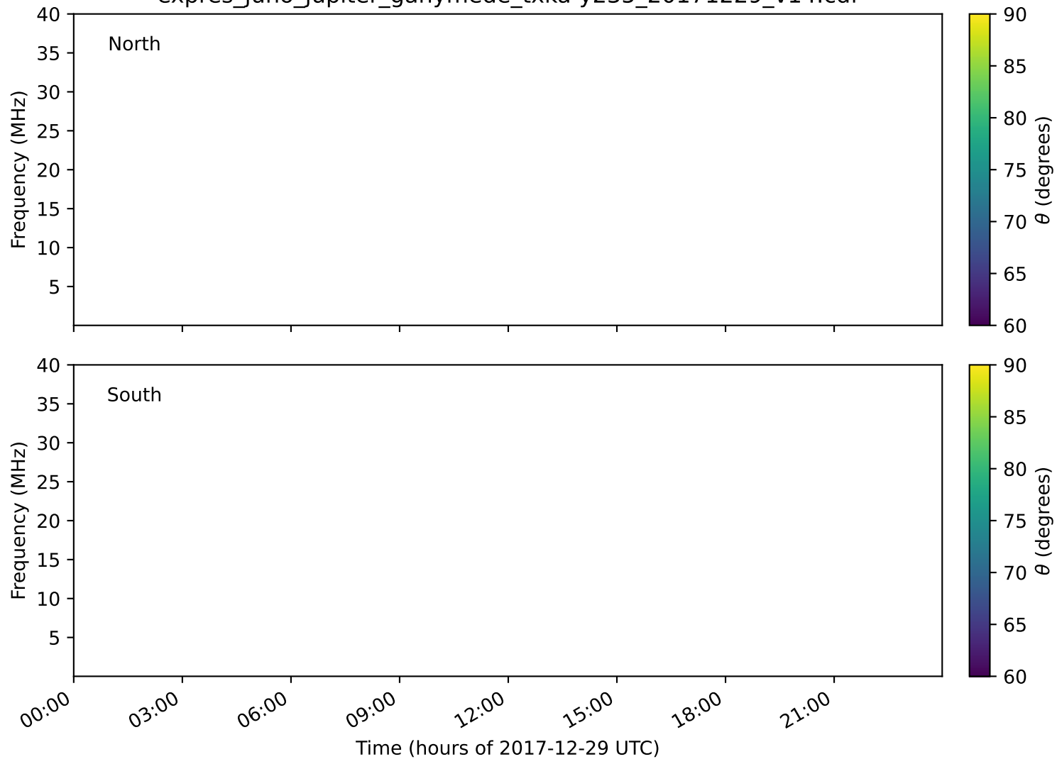
expres_juno_jupiter_ganymede_txka-y235_20171229_v14.cdf
