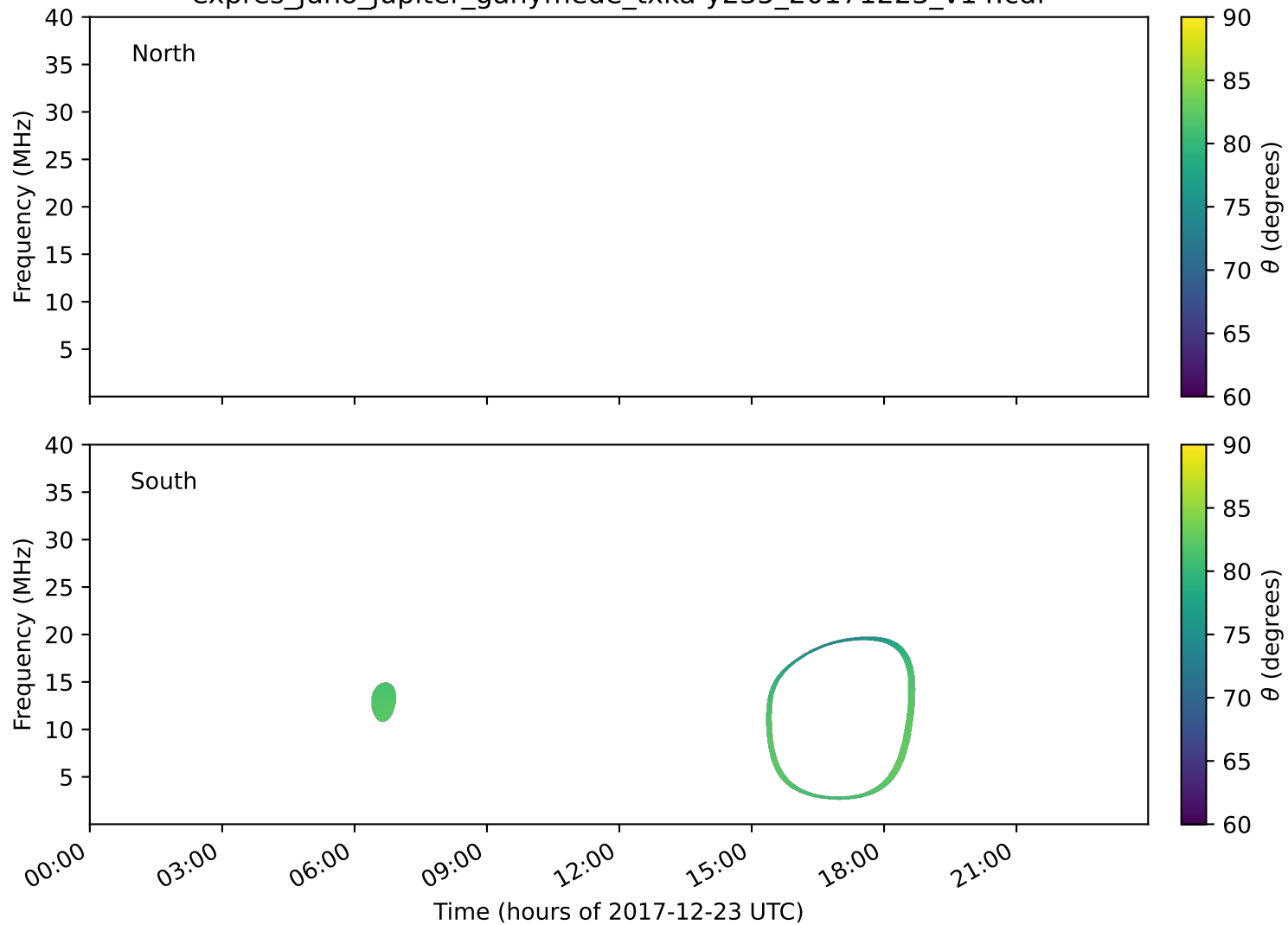
expres_juno_jupiter_ganymede_txka-y235_20171223_v14.cdf
