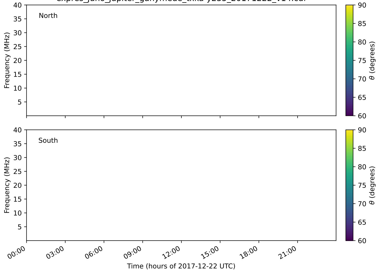
expres_juno_jupiter_ganymede_txka-y235_20171222_v14.cdf
