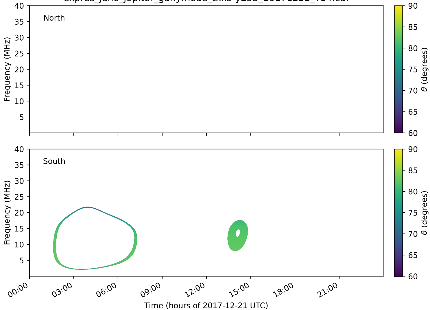
expres_juno_jupiter_ganymede_txka-y235_20171221_v14.cdf
