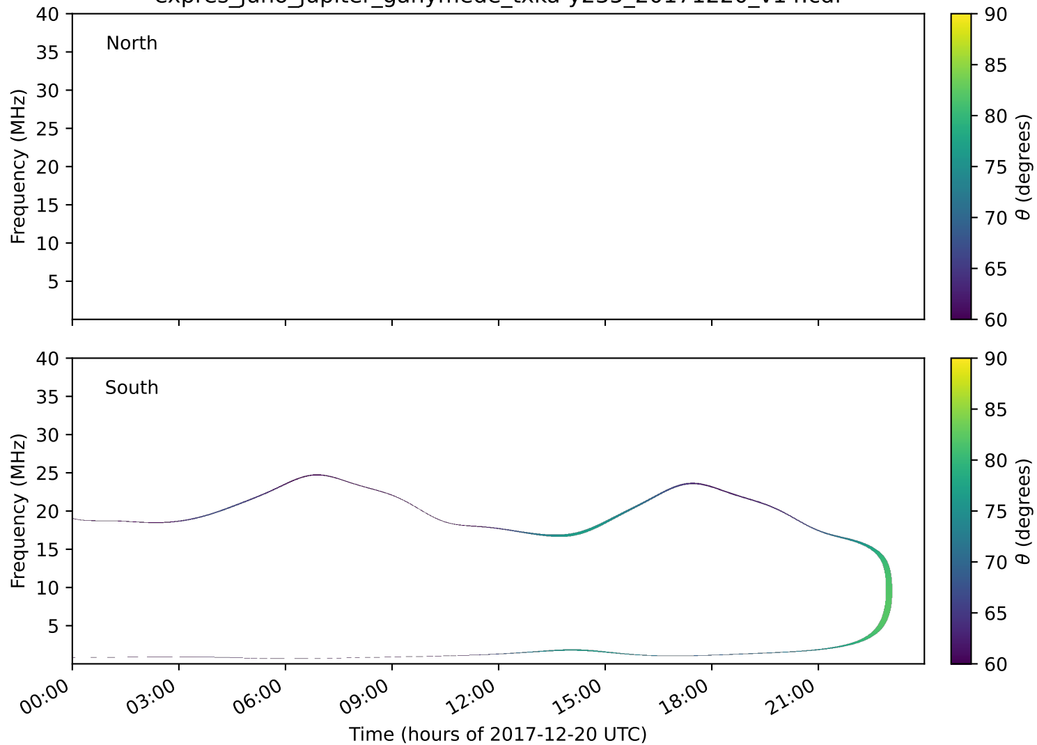
expres_juno_jupiter_ganymede_txka-y235_20171220_v14.cdf
