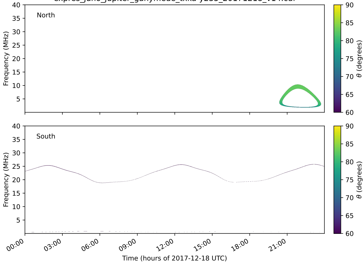
expres_juno_jupiter_ganymede_txka-y235_20171218_v14.cdf
