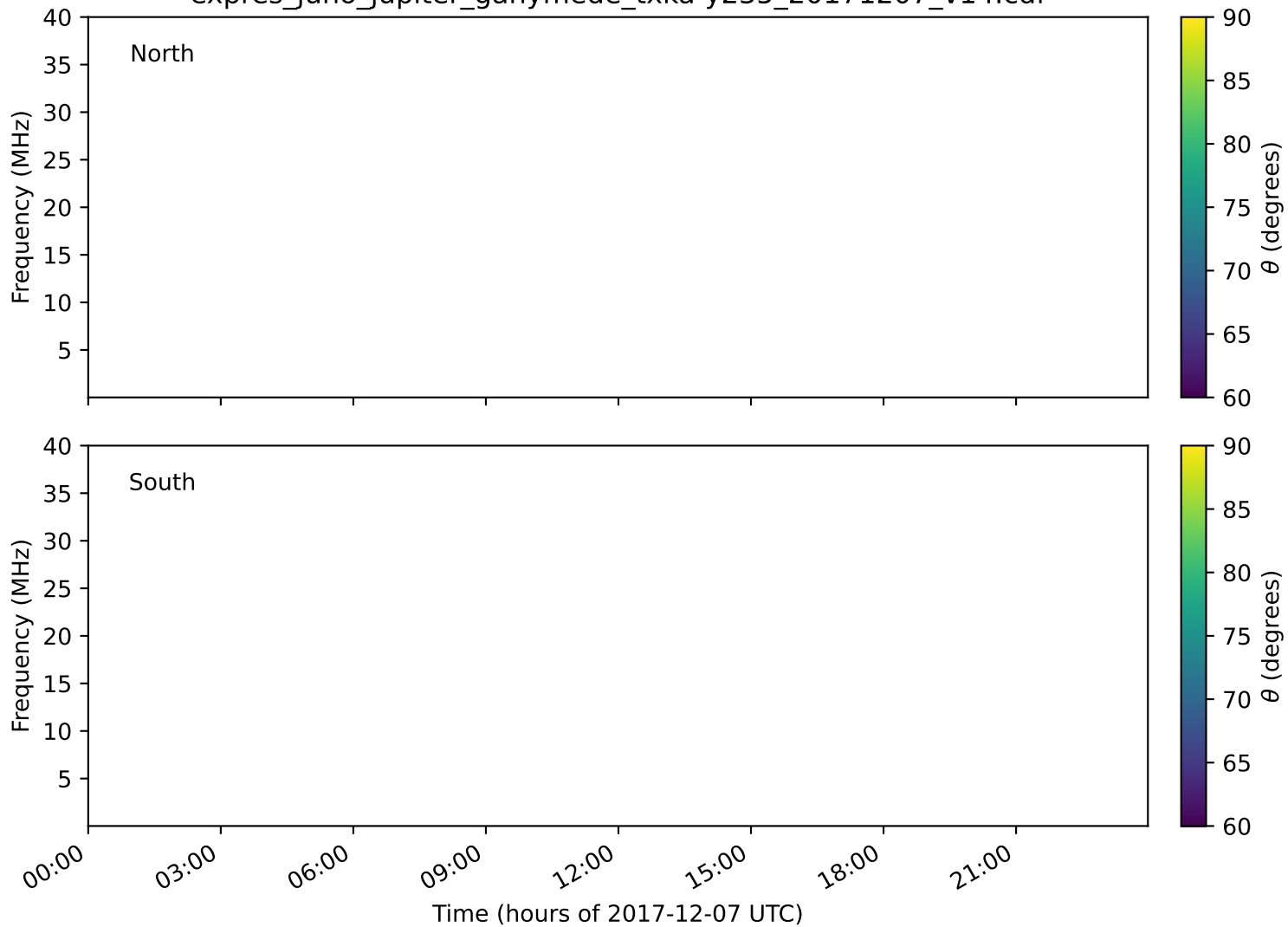
expres_juno_jupiter_ganymede_txka-y235_20171207_v14.cdf
