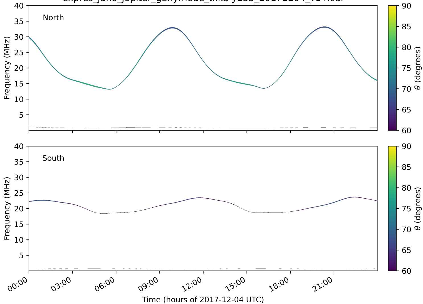
expres_juno_jupiter_ganymede_txka-y235_20171204_v14.cdf
