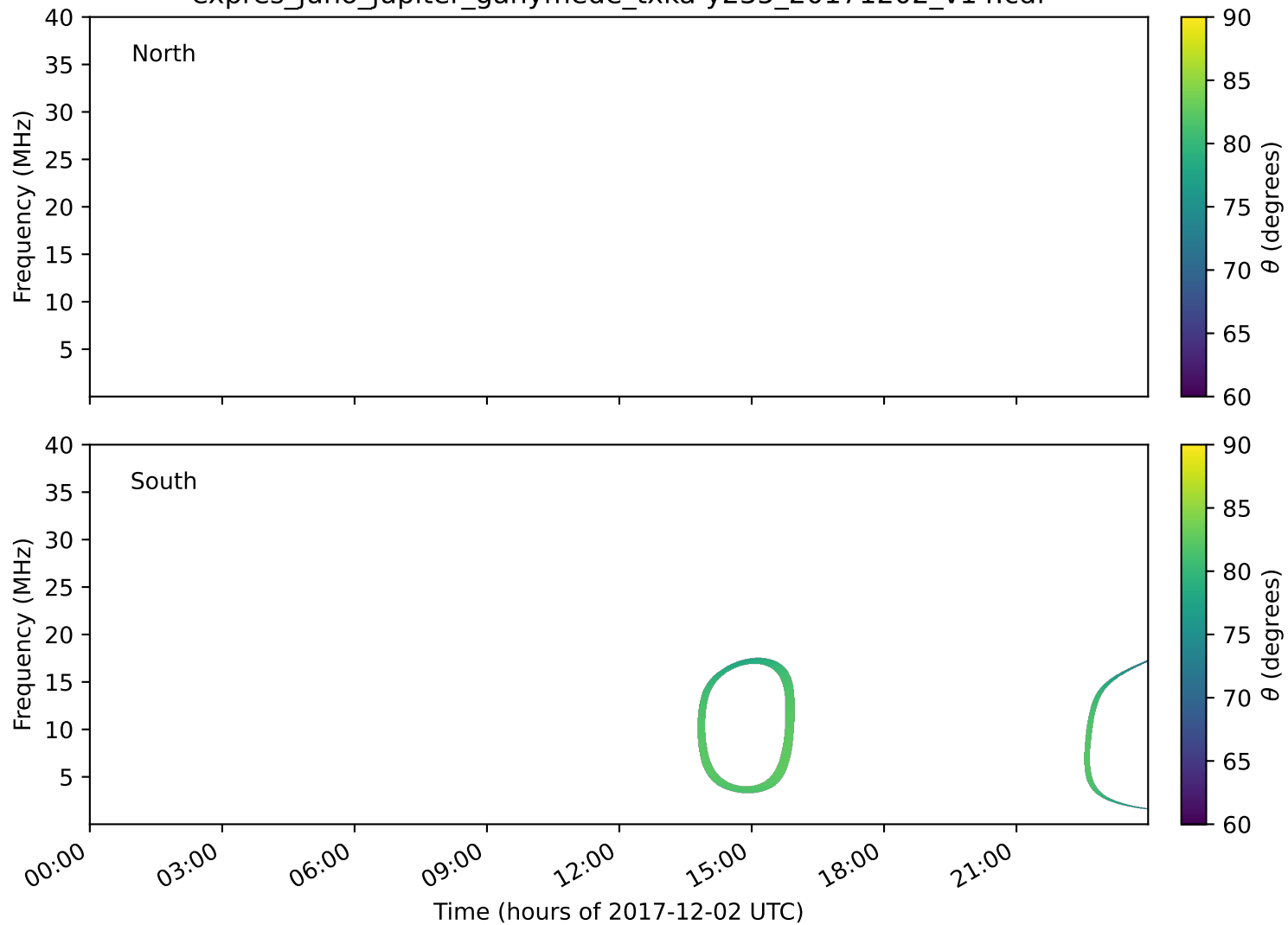
expres_juno_jupiter_ganymede_txka-y235_20171202_v14.cdf
