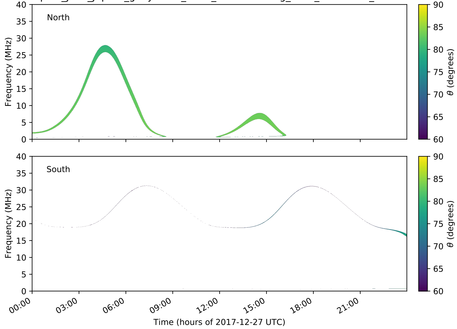
expres_juno_jupiter_ganymede_isaac_lossc-wid1deg_3kev_20171227_v01.cdf
