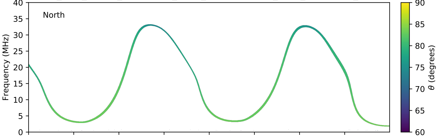
expres_juno_jupiter_ganymede_isaac_lossc-wid1deg_3kev_20171226_v01.cdf
